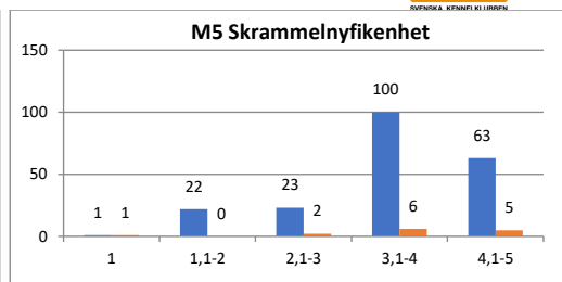
Diagram 13. Moment 5 "Skrammelnyfikenhet"
